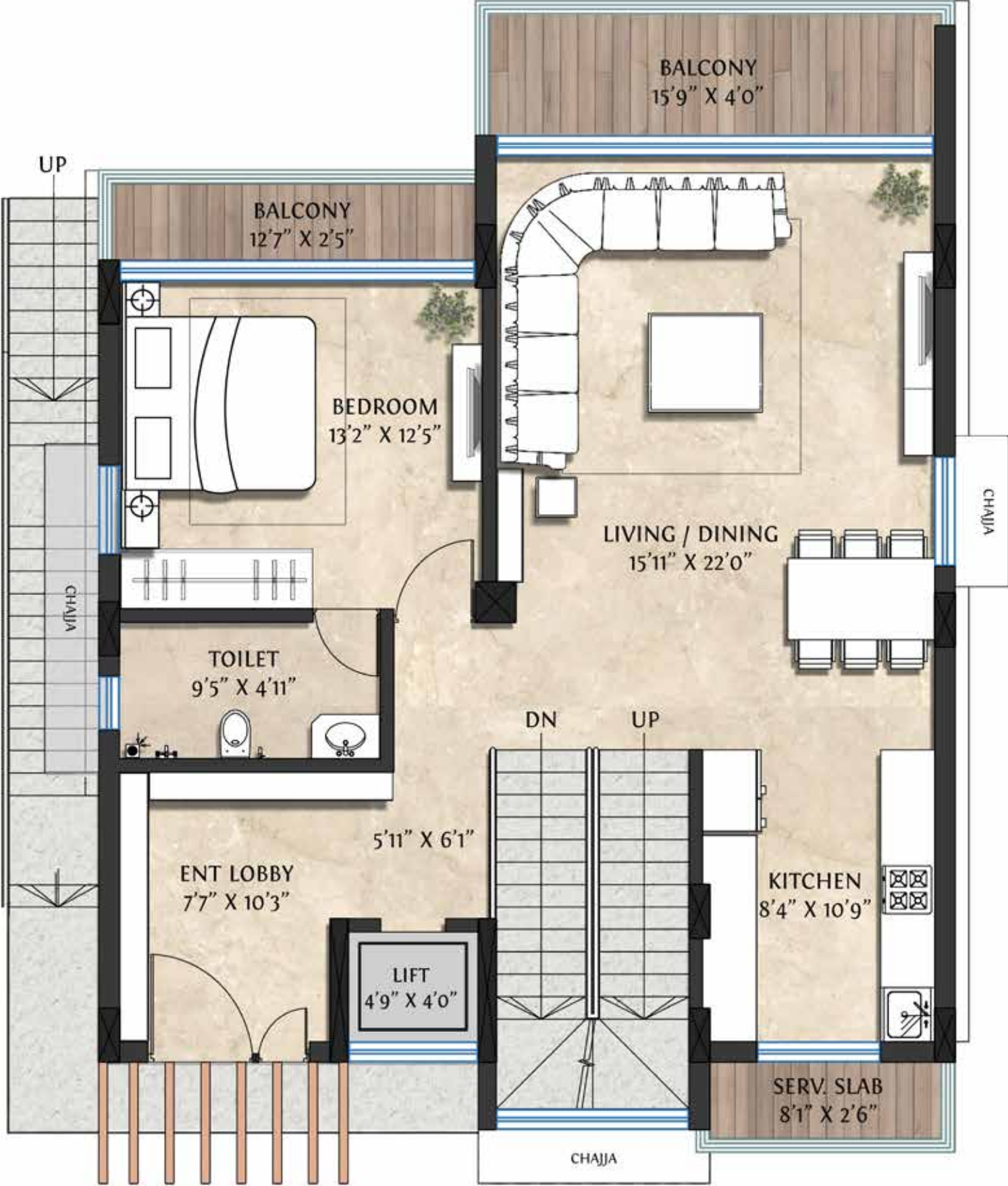
UPPER GROUND FLOOR PLAN
